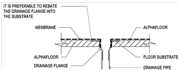
FIGURE 8: MEMBRANE TERMINATION AT DRAINAGE FLANGE
