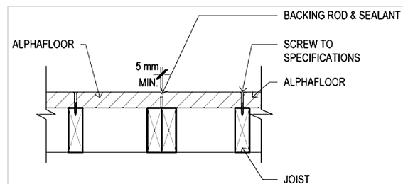
FIGURE 9: CONTROL JOINT AT PANEL END
