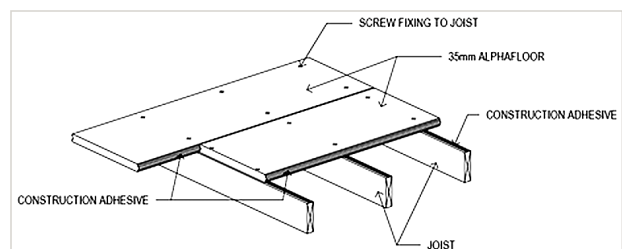
FIGURE 15: ALPHAFLOOR COMPONENTS
