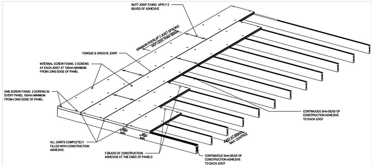
FIGURE 1: ALPHAFLOOR CONFIGURATION
