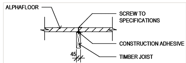
FIGURE 5: ALPHAFLOOR® FIXING TO TIMBER JOISTS
