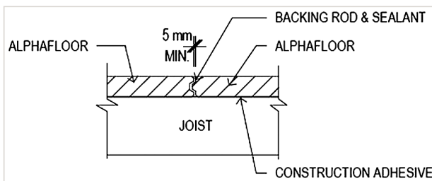
FIGURE 10: CONTROL JOINT AT PANEL EDGE
