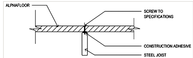
FIGURE 7: ALPHAFLOOR® FIXING TO STEEL JOISTS
