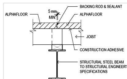
FIGURE 15: ALPHAFLOOR COMPONENTS
