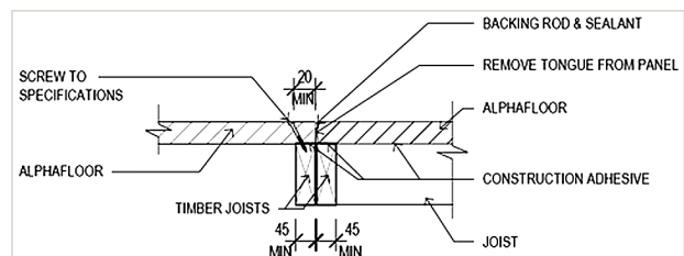
FIGURE 11: ALPHAFLOOR® FIXING AT END OF PANELS TO TIMBER JOISTS*
