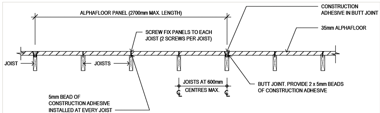
FIGURE 3: FLOOR SECTION - PERPENDICULAR TO JOISTS
