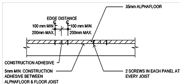
FIGURE 4: FLOOR SECTION - PARALLEL TO JOISTS
