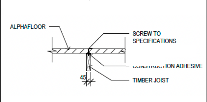
FIGURE 5: ALPHAFLOOR® FIXING TO TIMBER JOISTS
